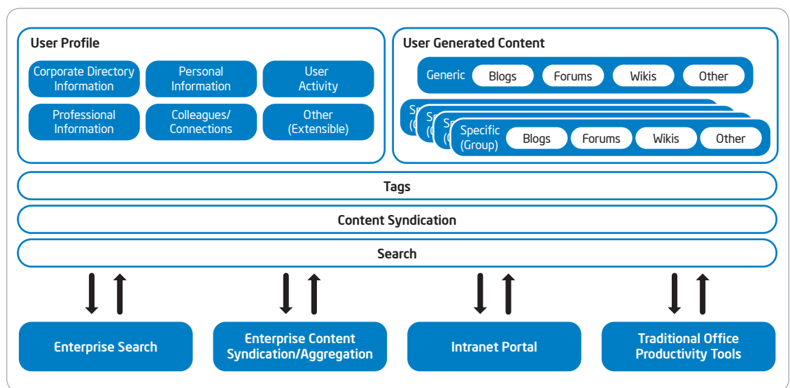
Figure 1. Social computing architecture.
